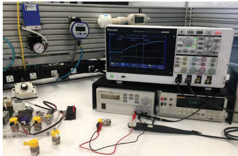
ABOVE: Performing helium leak detection test; BELOW: Custom testing station
